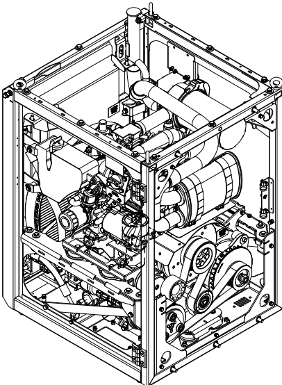
TURNED REAR ISOMETRIC VIEW
