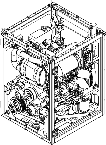
RIGHT HAND ISOMETRIC VIEW
